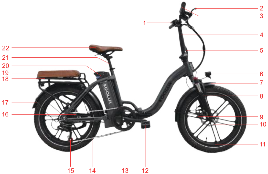
Figure 1 (Whole vehicle diagram)
